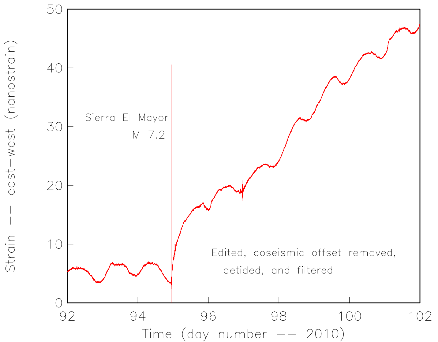
Earth Strain -- Pinon Flat -- Baja California Earthquake
