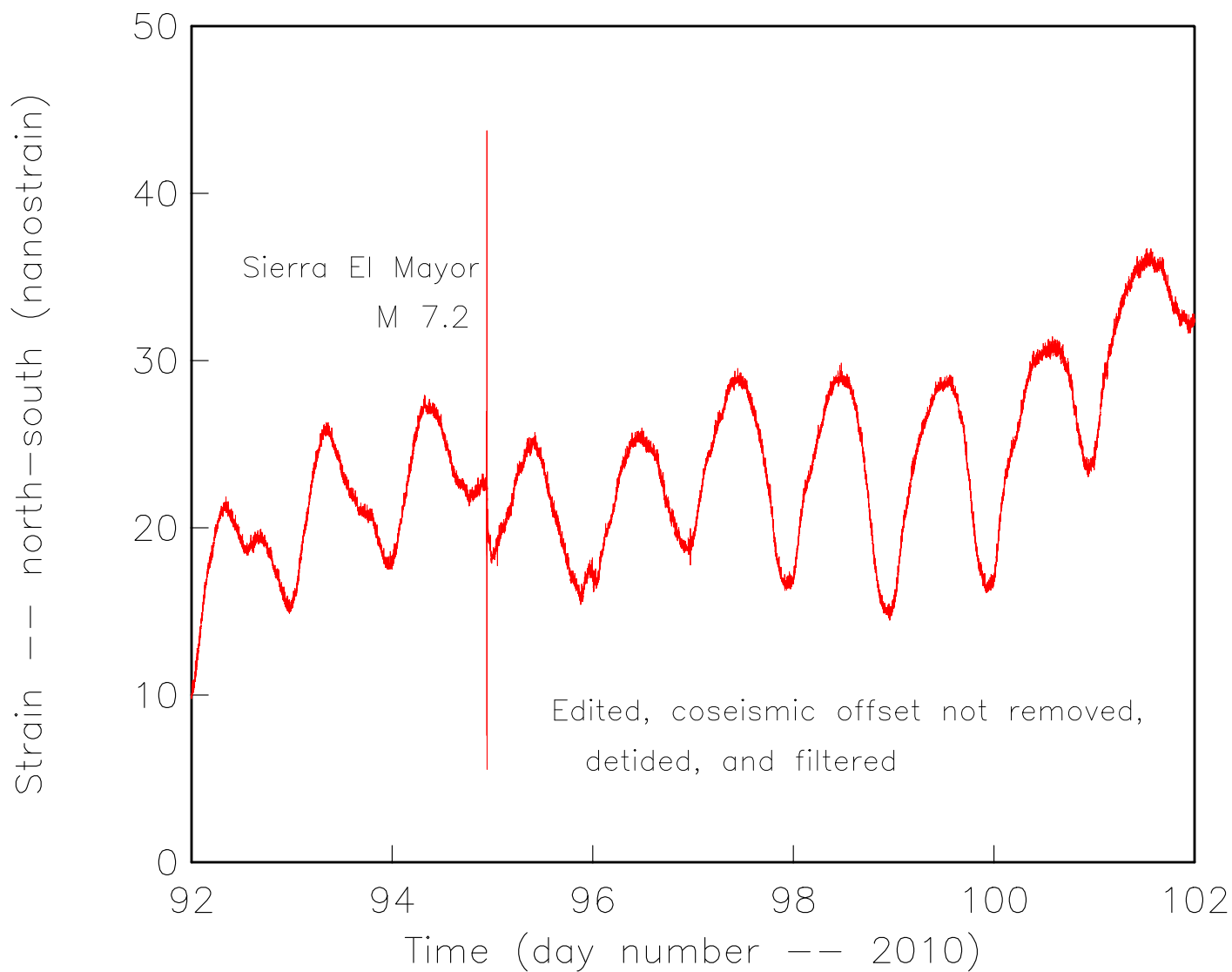
Earth Strain -- Glendale -- Baja California Earthquake
